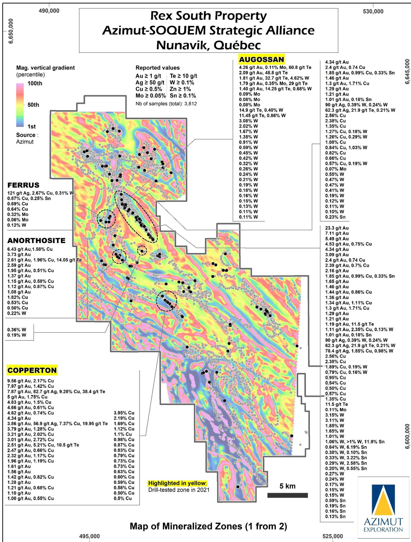
Figure 15: Map of the Rex South Property showing some of the significant zones and best grab samples (more in next figure).
