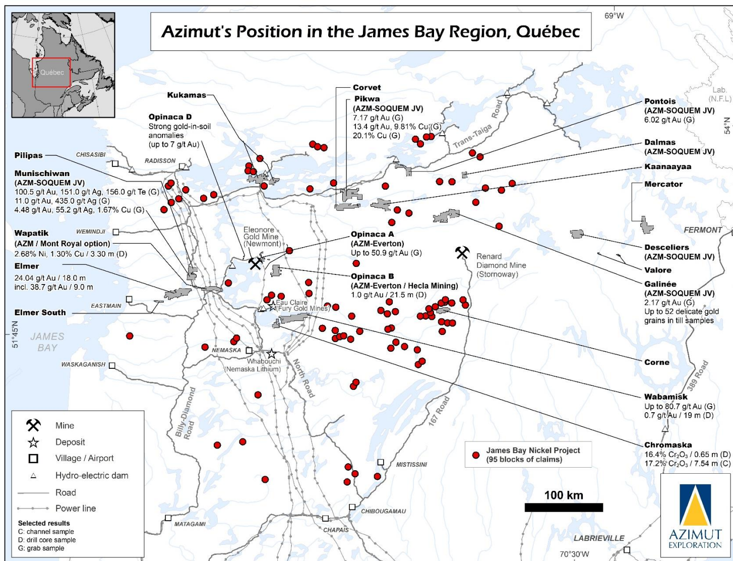
Figure 2: The Company's project portfolio in the James Bay region showing key results as at December 22, 2022.
