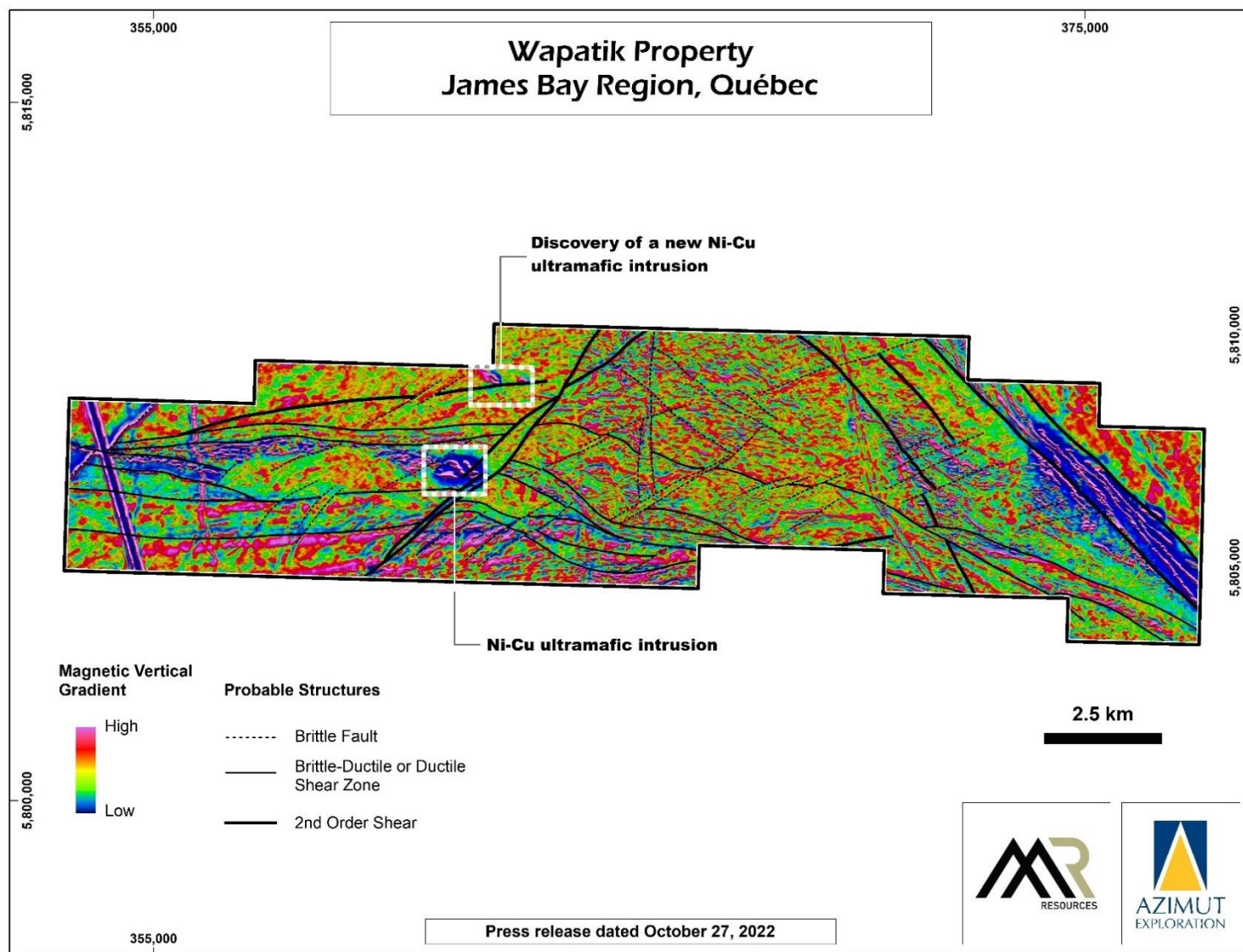
Figure 9: Magnetic map of the Wapatik Property showing structures and the locations of known mineralized intrusions.
