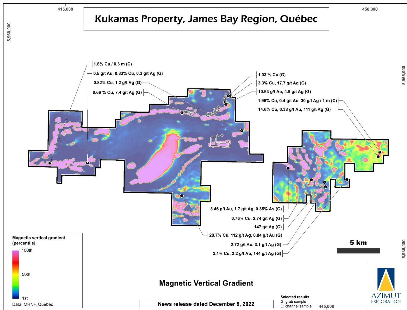
Figure 12: Magnetic map of the Kukamas Property showing historical grab samples.
